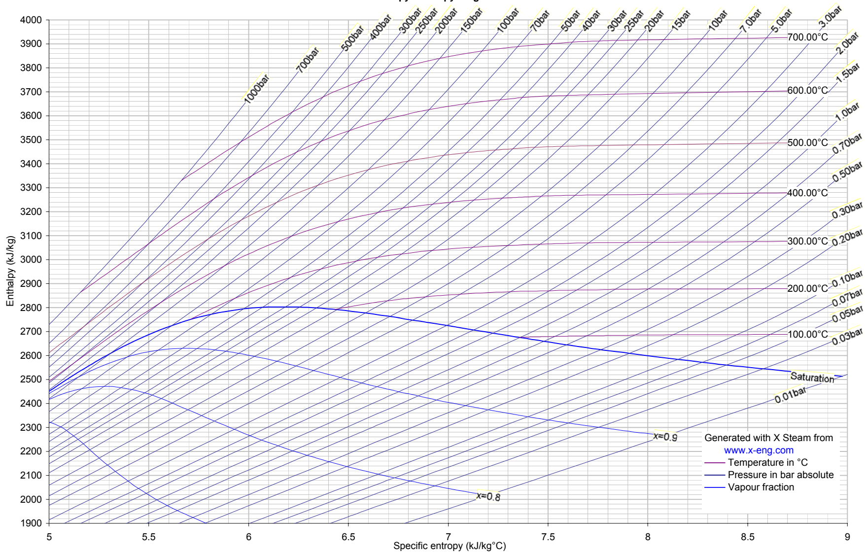
Enthalpy / Entropy Diagram
